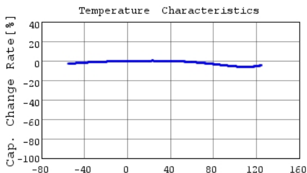
GRM155R71H682KA88 C-Temp. capchange, DC0.0V,
