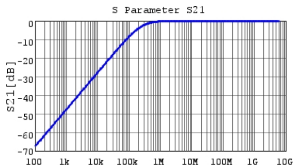
GRM155R71H682KA88 S21 DC0V, 25degC
