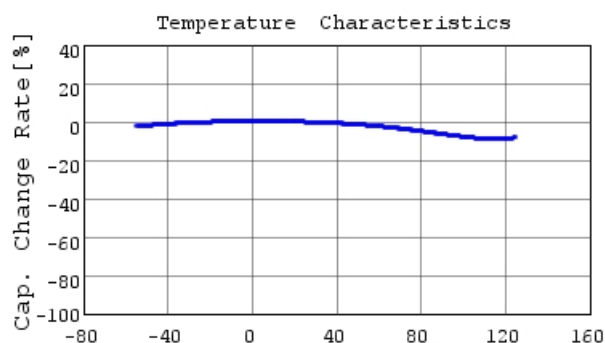
GRM155R71H153KA12 C-Temp. capchange, DC0.0V,
