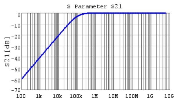
GRM155R71H153KA12 S21 DC0V,25degC
