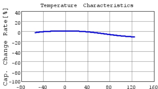
GRM155R71C683KA88 C-Temp. capchange, DC0.0V,
