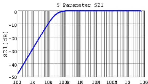
GRM155R71C683KA88 S21 DC0V,25degC
