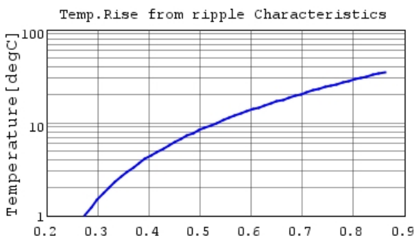
■ GJM1555C1H1R6BB01 Temp.rise 3GHz
