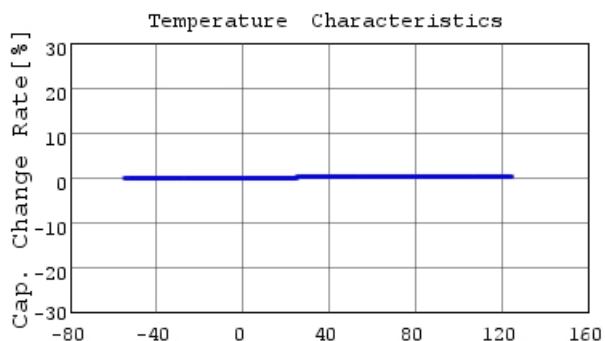
■ GJM1555C1H1R1BB01 C-Temp. capchange, DCOV, 1
